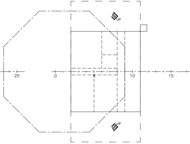
DECKHOUSE TOP DECK / HELIDECK
