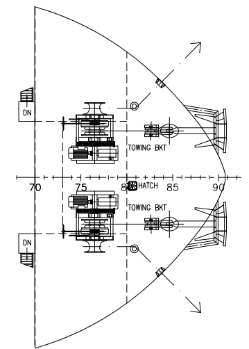
FORE CASTLE DECK
