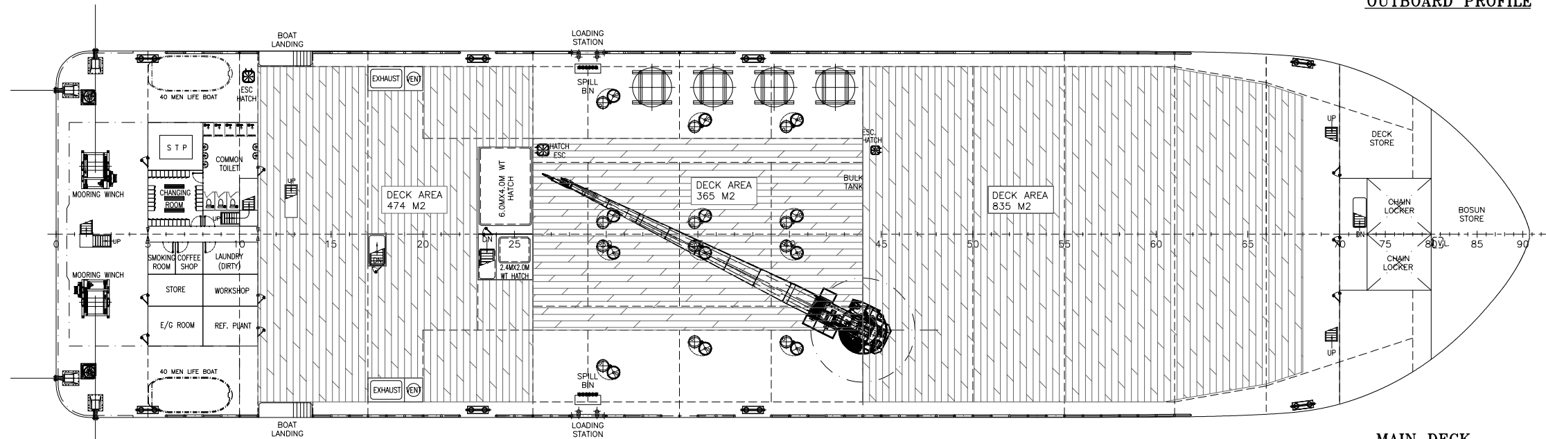
MAIN DECK
