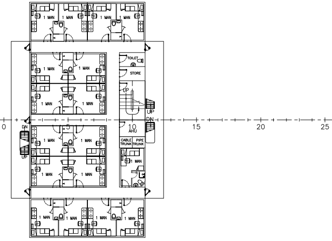
2nd DECK 1 MAN x 17 ROOMS = 17 MEN
