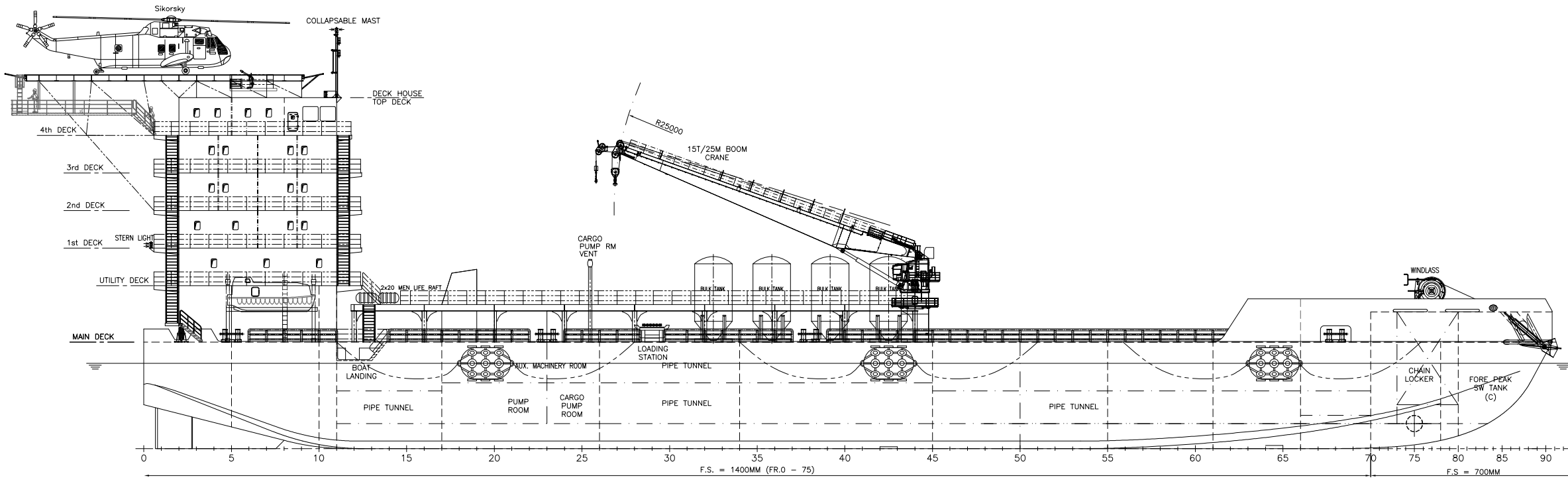
OUTBOARD PROFILE
