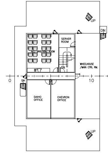
4th DECK
