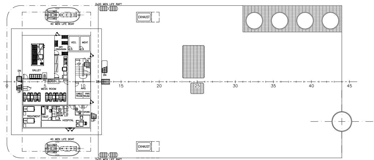
UTILITY DECK
