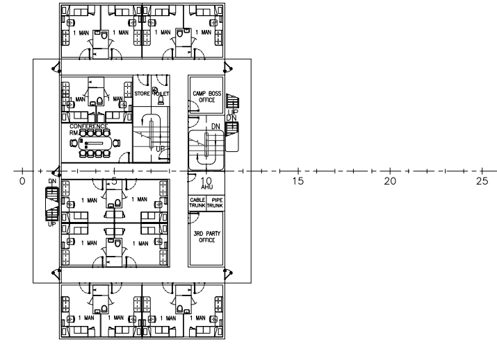
3rd DECK 1 MAN x 14 ROOMS = 14 MEN
