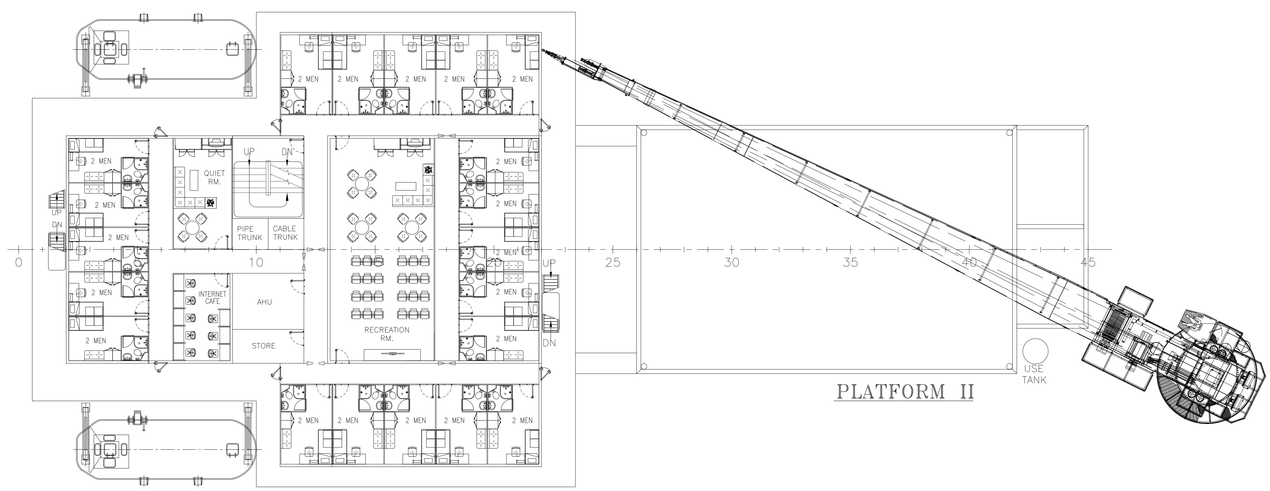
1st DECK
