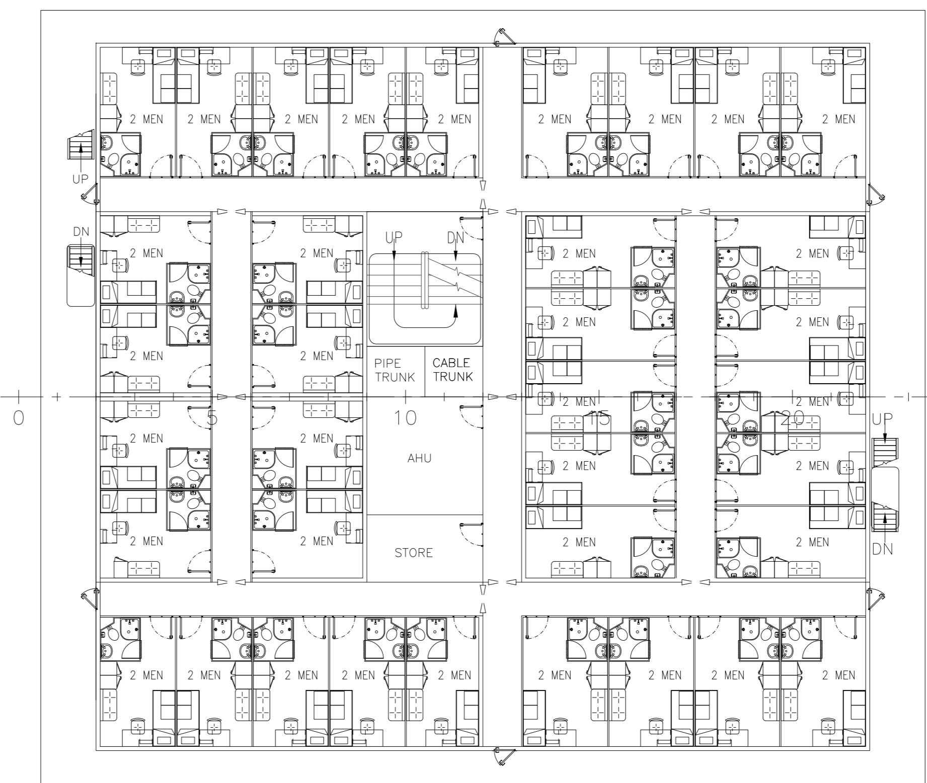
2nd DECK
