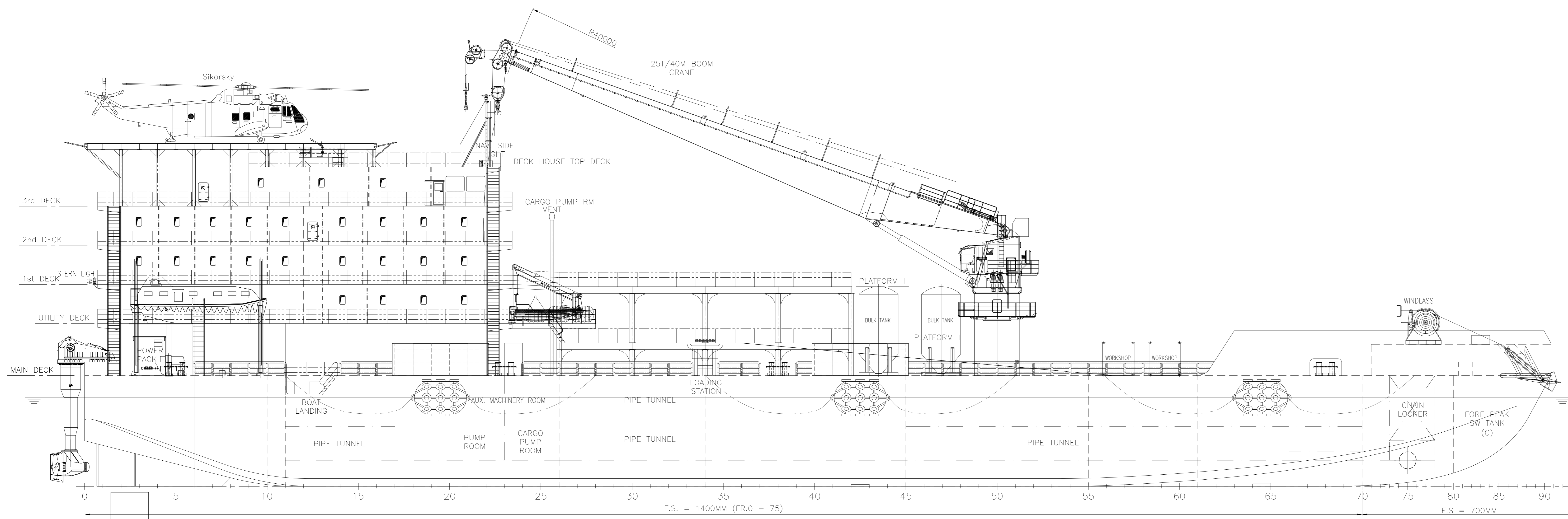
OUTBOARD PROFILE
