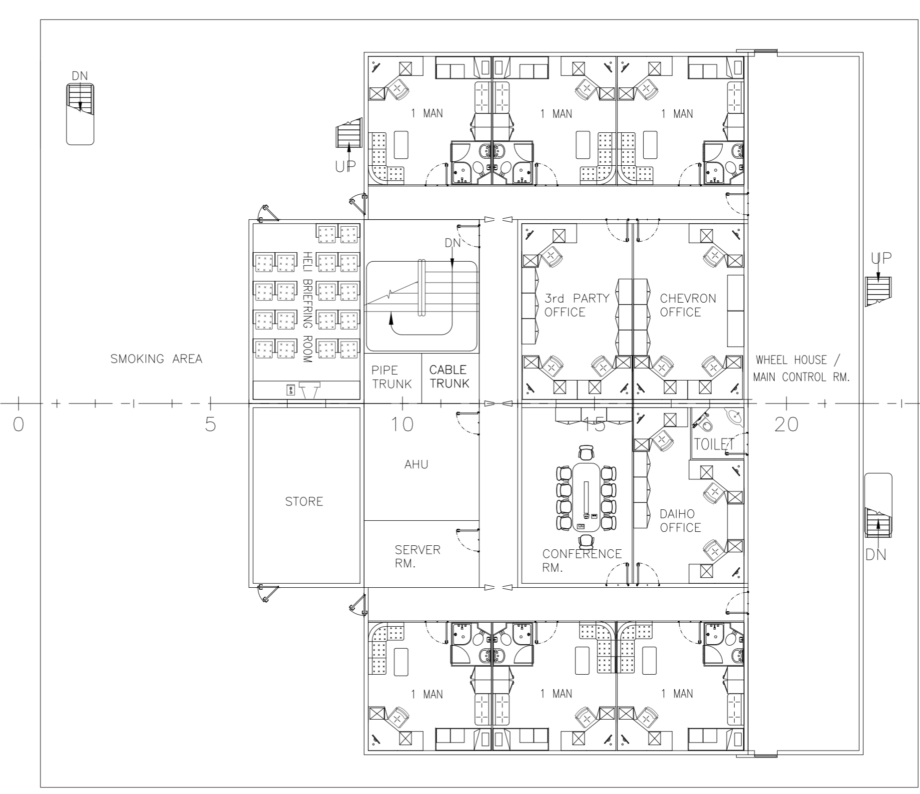
3rd DECK
